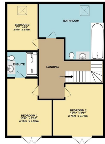
2ND FLOOR 794 sq.ft. (73.8 sq.m.) approx.
